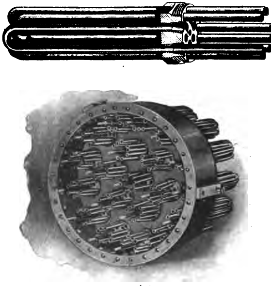
FIG. 163 —The Rider Tube Plug Water-tube Boiler, showing one tube plug and the assembled boiler.
